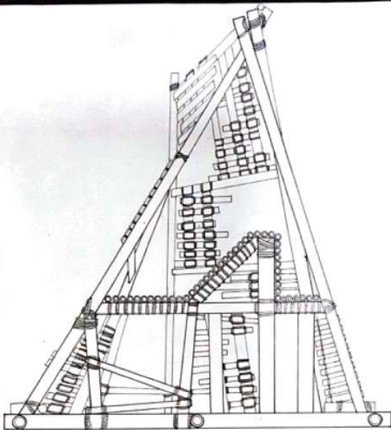
ELEVATION VIEW SCALE 1:10
